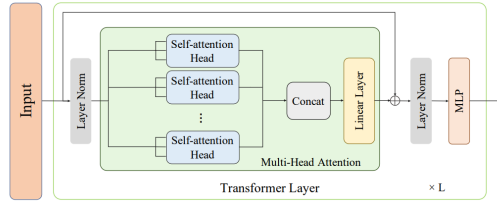
Figure 2.5 An illustration of a Transformer layer that is used in RADIANT
