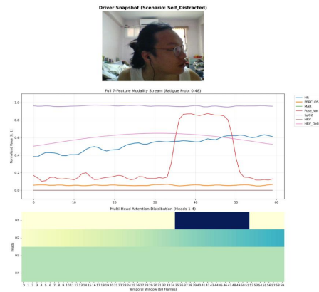
Figure 4.9 7-Feature Case Study.
